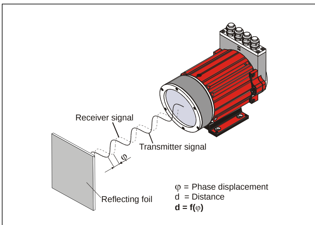
Figure 1: Function principle
