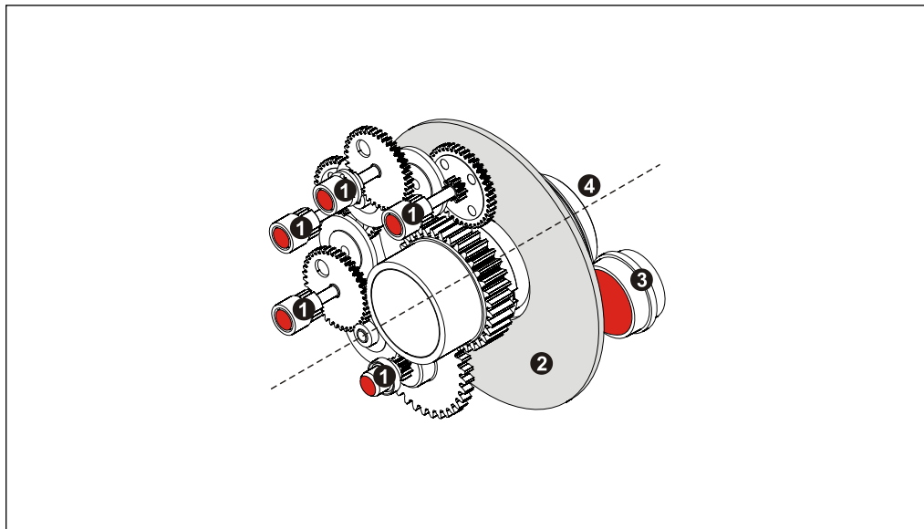
Figure 1: Measuring system operating principle (single scanning)
