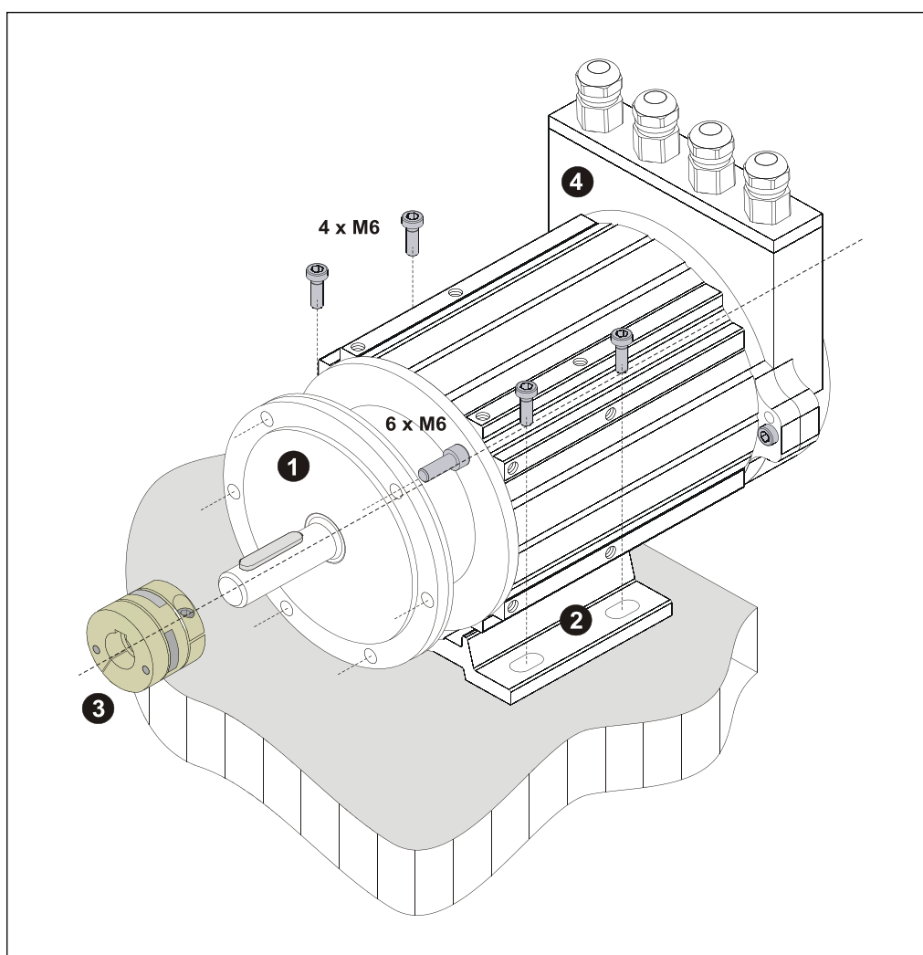
Figure 3: Mounting example
