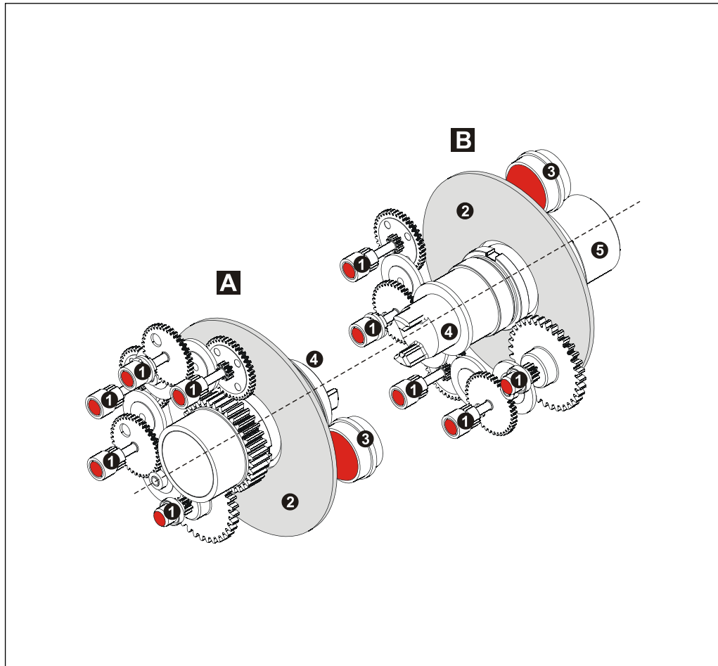
Figure 2: Measuring system operating principle (double scanning)
