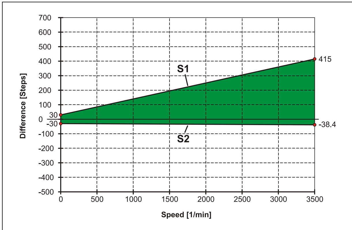
Figure 1: Dynamic view of the step deviation, counting direction rising (view onto flanging)
