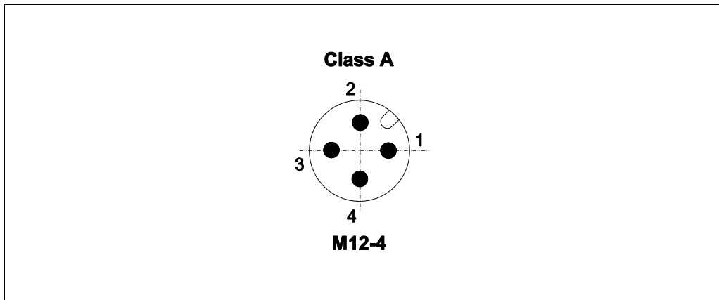
Figure 3: M12 male connector, A-coded
